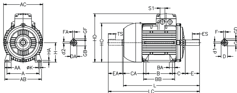
FRAME: 132M Current Design
