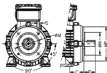
FRAMES: 71, 80, 90S/L, 100L, 112M* and 132S/M*
